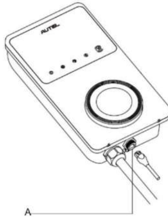
Figure 2-4 Connexion du câble RJ45
